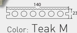
Code: SU140x23 Size : 2400mm x 140mm x 23mm Finished Surface: Ultrashield
